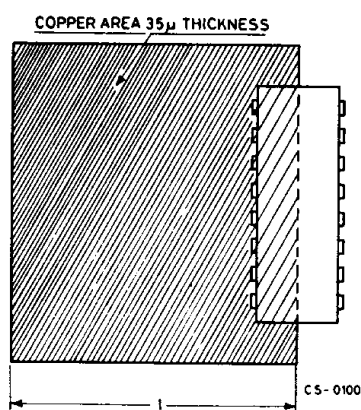
Figure 21. Example of heatsink using PC board copper ( l = 65\text{ mm} )
