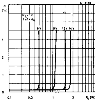
Figure 10. Distortion vs. output power
